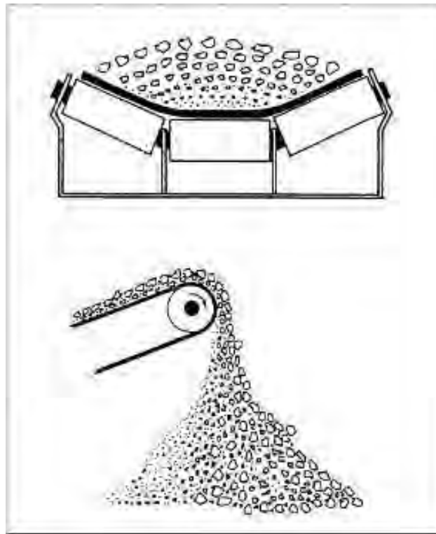
Figure 7-8. Belt segregation.
