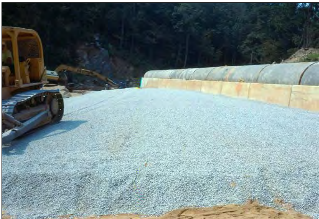
Figure 2-10. Gravel blanket drain being placed over fine filter shown in Figure 2-9. (Photo courtesy of NRCS, Alabama.)
