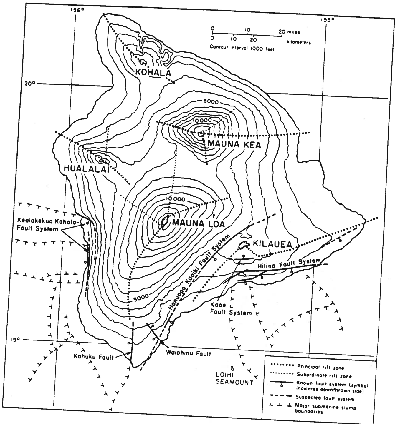
Figure 11. Map showing volcanic rift zones and faults on the island of Hawaii. (In Macdonald et al., 1983; submarine slumps after Normark et al., 1978)
