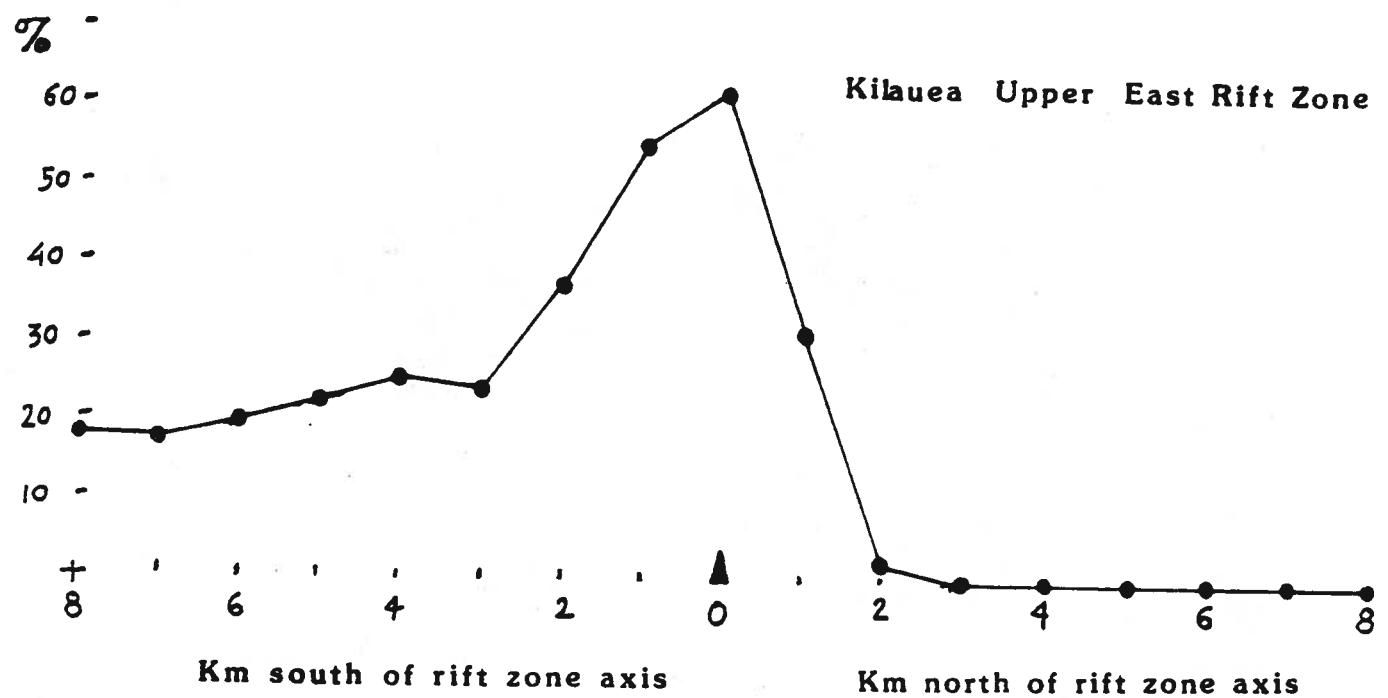
Figure 10. Percentage of ground covered by lava flows, from 1954 to 1984, as it varies with distance north and south of Kilauea's east rift zone axis. If 30 years is the assumed life of a geothermal power plant, these figures suggest the probability that sites may be threatened by burial during their lifetime, as based on Kilauea's history from 1954 to 1984.
