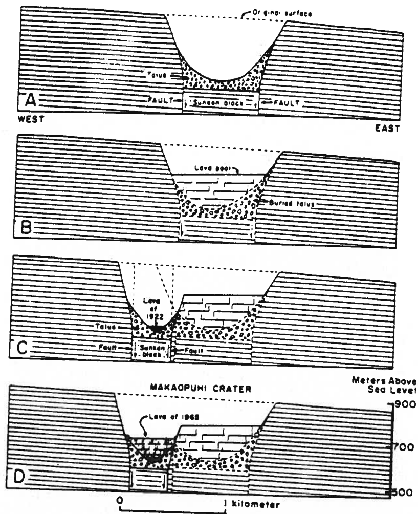
Diagram showing the manner of formation of Makaopuhi, a double pit crater. A. A subcircular fault block sinks, leaving a crater at the surface. (The position and attitude of the faults is hypothetical.) The upper walls of the crater collapse to form taluses (piles of rock fragments) that hide the lower walls. B. Lava pouring into the crater collects in a deep pool, the surface of which solidifies to form a nearly flat floor. C. A second block sinks, making a second crater that cuts across the western edge of the first one. The pool of lava in the bottom of the second crater is from a small eruption in 1922. D. A much larger eruption (in 1965) forms a pool 90 meters deep in the second crater. Note the slump scarps at the edge of the new lava floor, formed as lava in the central part of the crater drains back into underlying vents.
