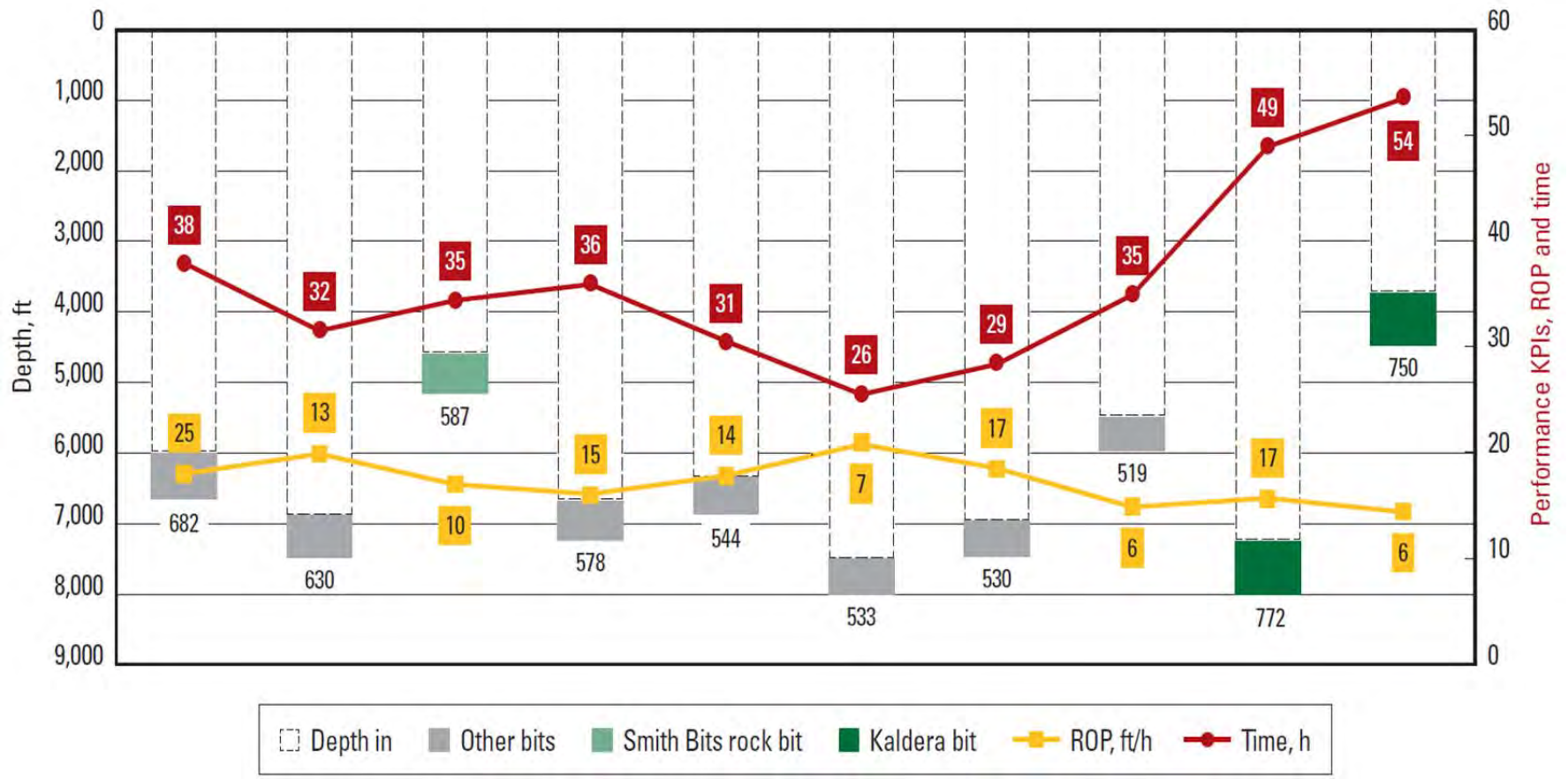
Figure 9.2: Kaldera drilling results at The Geysers: The Kaldera bit drilled 14 hours longer and approximately 150 feet farther than other bits, representing a run length increase of 25% (Schlumberger, 2013).
