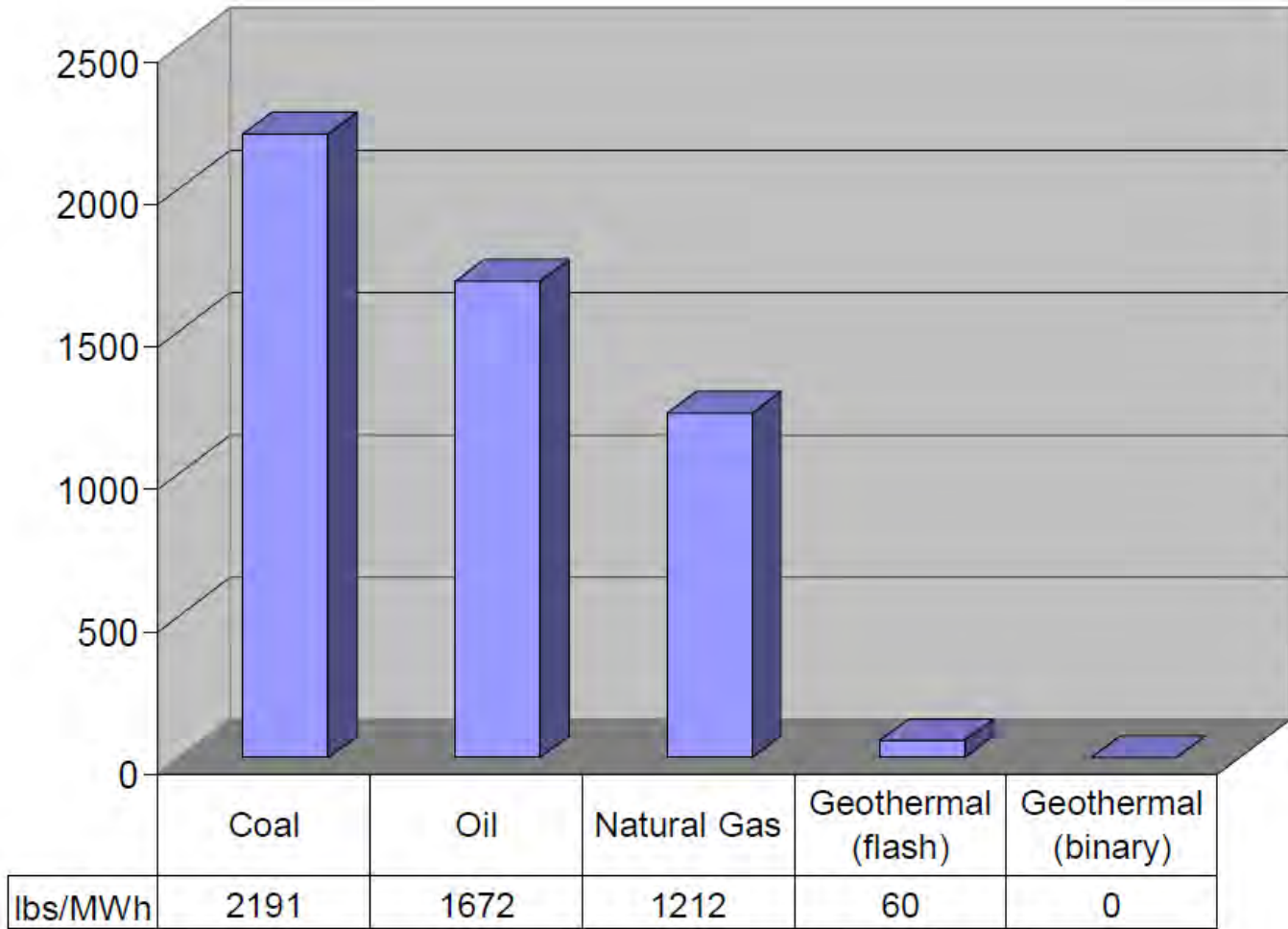
Figure 2.9: Relative output of CO 2 , expressed in pounds (lbs) per unit of energy (megawatt-hours, MWh) (GEA, 2007).
