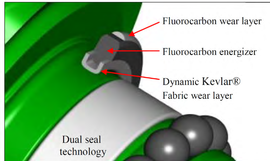
Figure 9.5: LEFT: Basic roller cone technology (top) and schematic of RC seal on journal bearing (bottom); RIGHT: New HT/HP seal packages in single configuration (top) and dual configuration (bottom) (Orazzini et al. , 2011).
